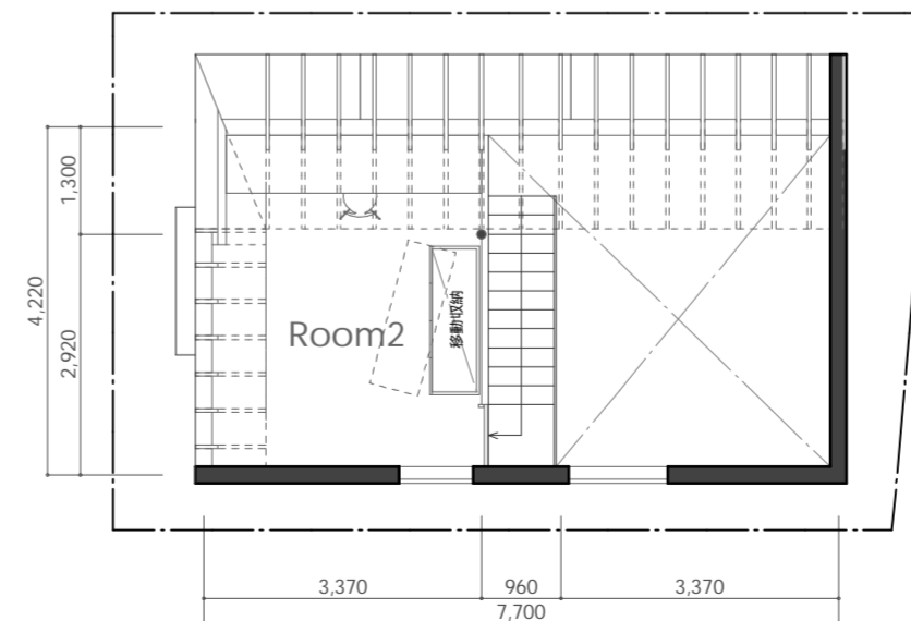
3F plan 1/100(A2)
