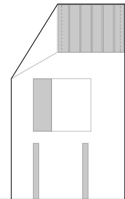
North-elevation 1/100(A2)
