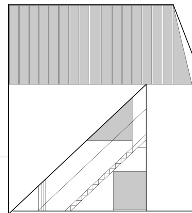
East-elevation 1/100(A2)
