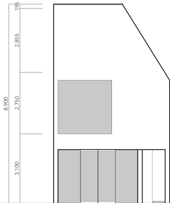
South-elevation 1/100(A2)
