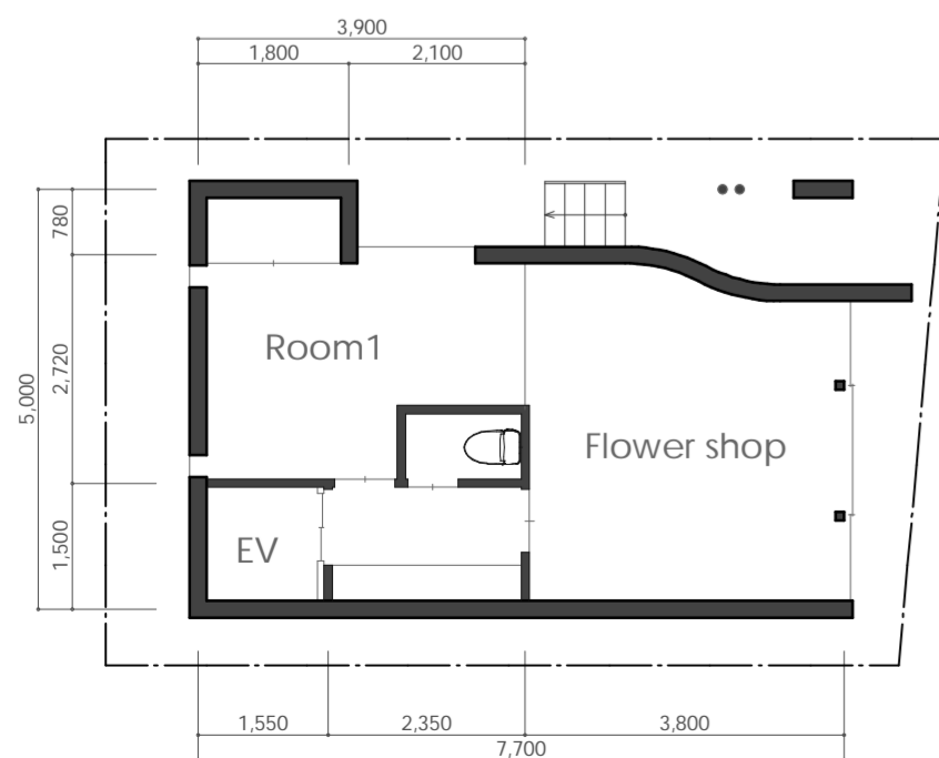
1F plan 1/100(A2)
