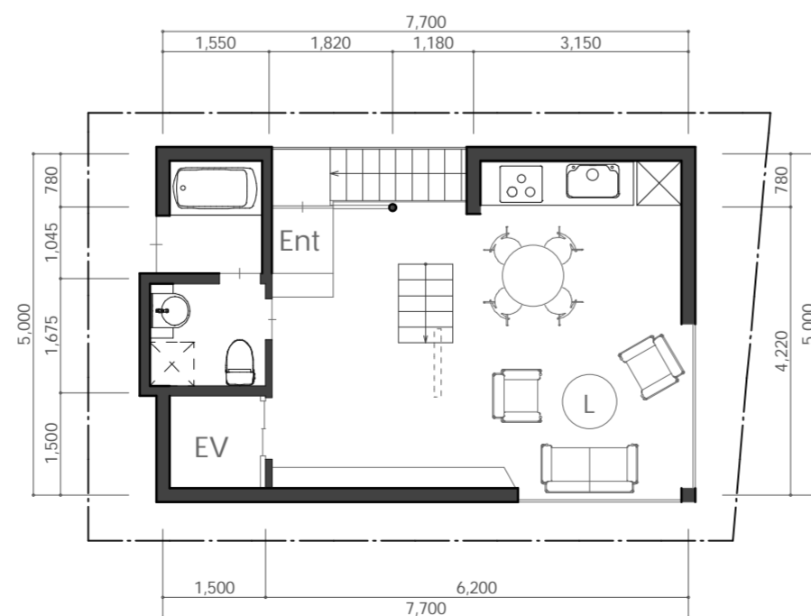
2F plan 1/100(A2)
